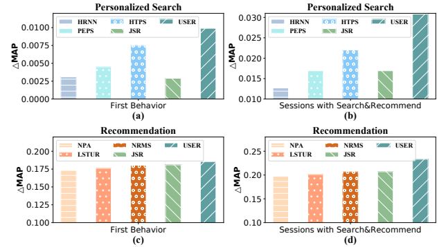
Figure 4: Performance on different data subsets. (a), (c): the first search/recommend behavior of each user; (b), (d): sessions with both search & recommendation.
